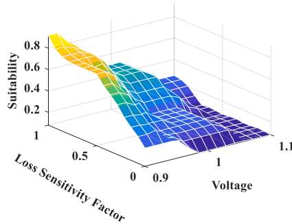
Fig. 5. The surface chart of fuzzy expert rules.
