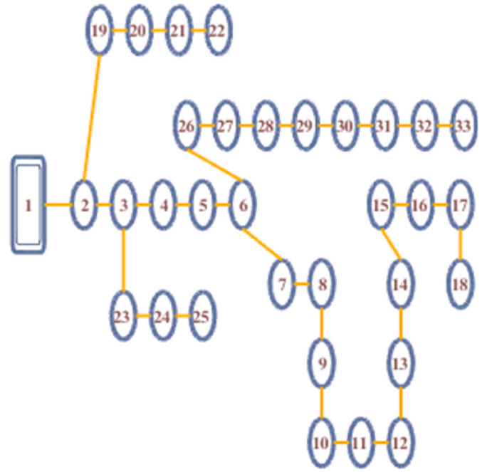
Fig. 8. Network layout of 33-bus RDN.
