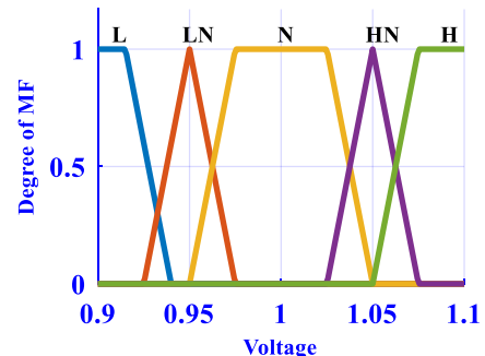
Fig. 2. MFs for voltage.
