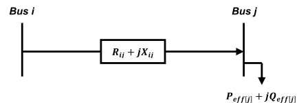
Fig. 1. A model of distribution line.
