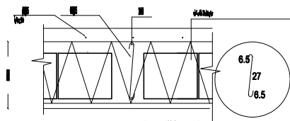
Section G-G
